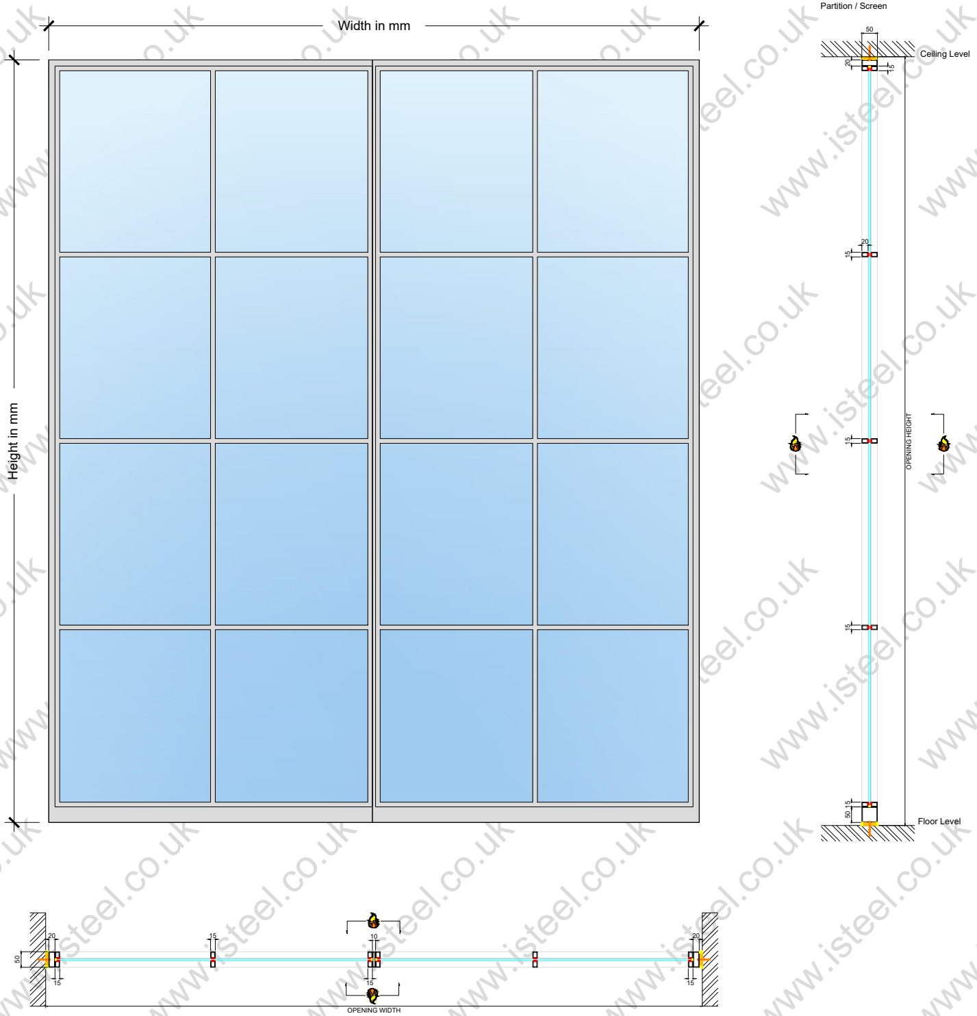
Plan Section
